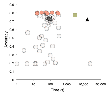
Figure 1 Accuracy score plotted against speed of contest-commissioned immunoglobulin sequence annotation code. Shown are the accuracy and speed (computational time) of 70 final submissions (top ten in red circles; remainder in unfilled circles), MegaBLAST (triangle) and in-house code (square) processing 100,000 in silico -generated recombined VDJ sequences. Accuracy score is the fraction of gene segment annotations that matched the corresponding gene segments used in generating the sequence. Note that because the sequence contains mutations, the best annotation might differ from the segment used, resulting in a maximum possible accuracy of <1.0 .
